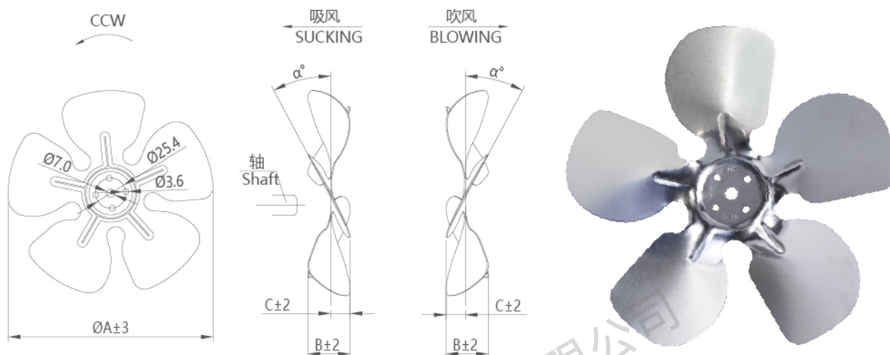
风叶规格尺寸 Fan specification and dimension
