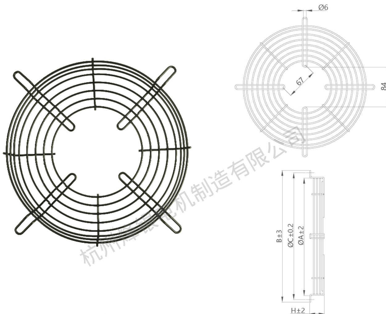
规格尺寸 Specification size
