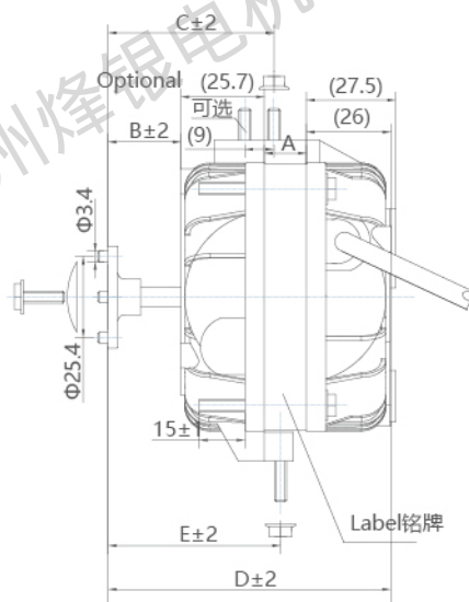
Model 型号 Rated voltage Rated frequency Input power Rated power Rated current Rated speed Air volume Fan blade Net weight Size尺寸 License 认证 额定电压 V 额定频率 Hz 输入功率 W 额定功率 W 额定电流 A 额定转速 r/min 额定风量 m³/h 风叶型号 mm 净重 kg A mm B mm C mm D mm E mm YZF48N-25W 220-240 50/60 25 3.5 0.145 1300 260 Ø170 0.8 13 15 43 79 46 CCC,CE 220-240 50/60 35 5 0.17 1300 450 Ø200 0.8 13 15 43 79 46 CCC,CE 110-120 60 35 5 0.4 1550 450 Ø200 0.8 13 15 43 79 46 YZF48N-40W 220-240 50/60 40 10 0.26 1300 650 Ø230 1.0 19 16 51 87 47 CCC,CE 110-120 60 40 10 0.53 1550 650 Ø230 1.0 19 16 51 87 47 YZF48N-60W 220-240 50/60 60 16 0.37 1300 900 Ø250 1.3 25 16 57 93 47 CCC,CE 110-120 60 60 16 0.65 1550 900 Ø250 1.3 25 16 57 93 47 YZF48N-75W 220-240 50/60 75 20 0.57 1300 1000 Ø254 1.6 30 15 61 97 46 CCC,CE 110-120 60 75 20 1.1 1550 1000 Ø254 1.6 30 15 61 97 46 YZF48N-90W 220-240 50/60 90 25 0.6 1300 1100 Ø300 1.9 40 14 70 106 45 CCC,CE 110-120 60 90 25 1.4 1550 1100 Ø300 1.9 40 14 70 106 45 YZF48N-110W 220-240 50/60 110 34 0.85 1300 1100 Ø300 2.2 45 14 70 112 45 CCC,CE 110-120 60 110 34 1.5 1550 1100 Ø300 2.2 45 14 70 112 45
