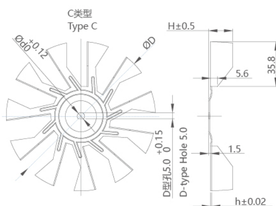
风叶规格尺寸 Fan specification and dimension
